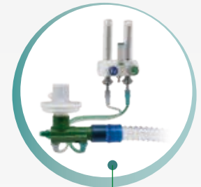
Venturi-effect flow generator COMPACT model, complete with corrugated tube, usable with any model of CPAP helmet (flow meter optional).
